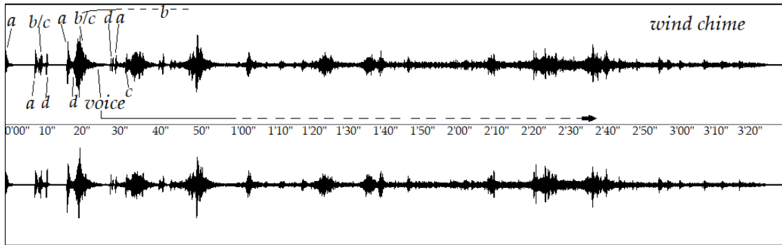
Figure 3: Sonogram, 0'00''- 3'33''
